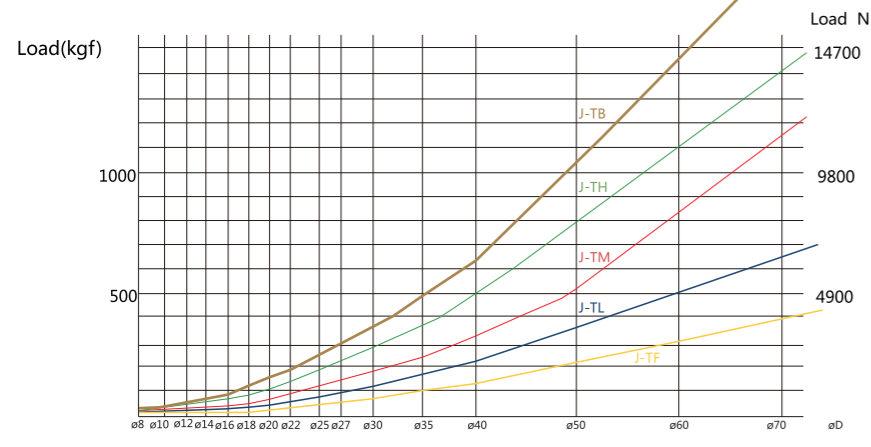
Numbers of bend: 0.3 million bend 30万次
